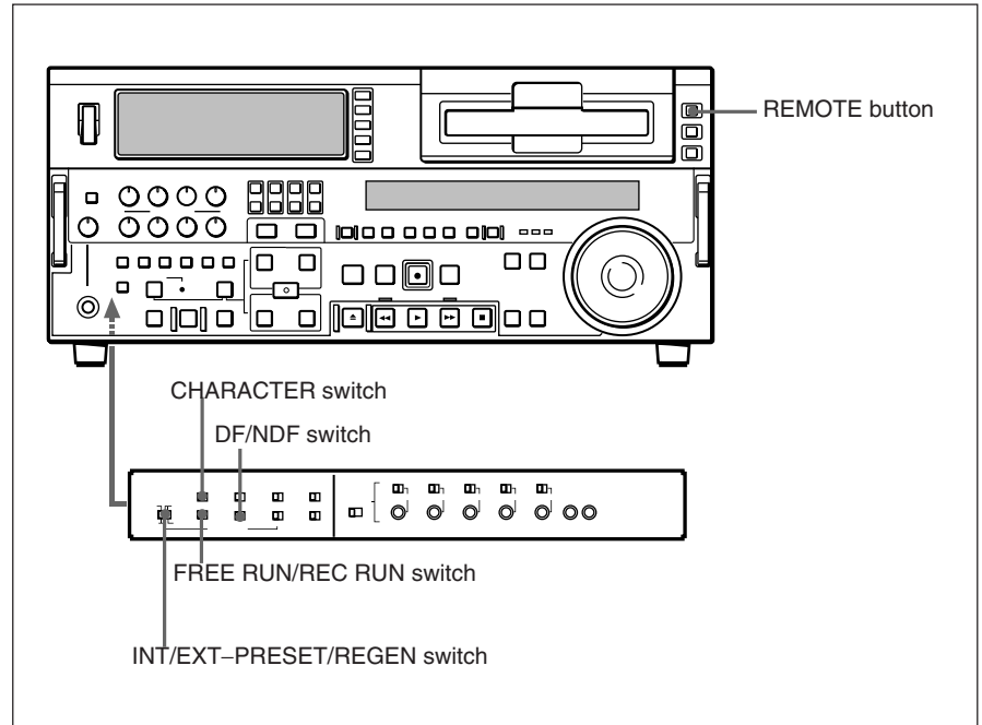
Button/switch settings
